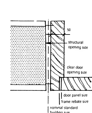
⑦ Full lining door frame (UK)
